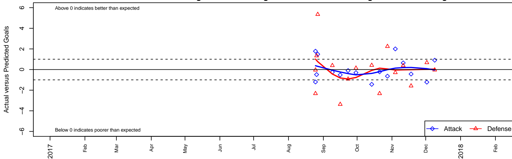
Washington United G04 Dots are actual minus expected GF (blue circles) and GA (red triangles). Blue line is smoothed change in attack strength. Red is smoothed change in defense strength.
